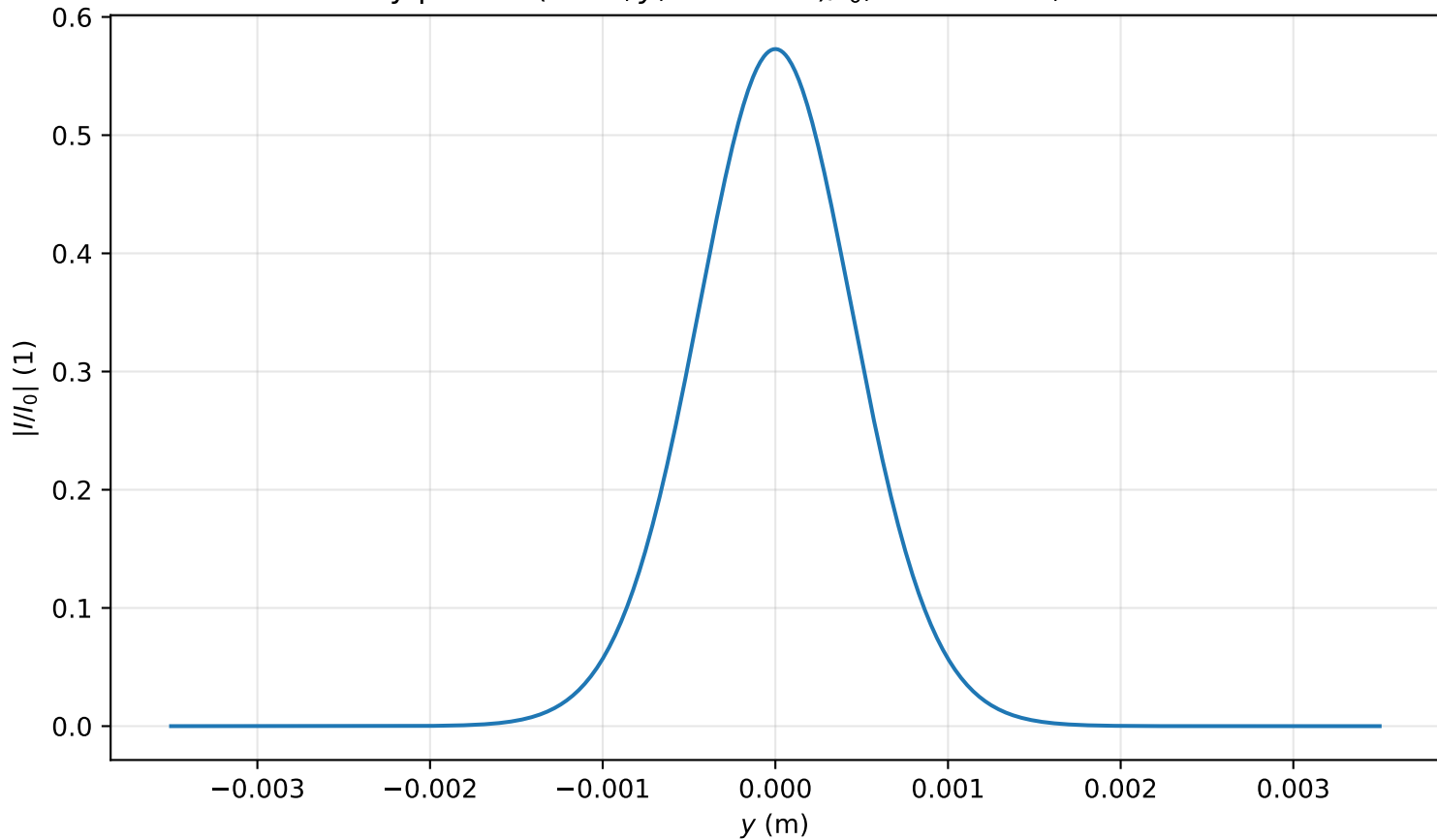
Intensity profile I(x=0, y, z=2.070)/I_0 , P_{in}=0.2P_{cr} , artificial time
